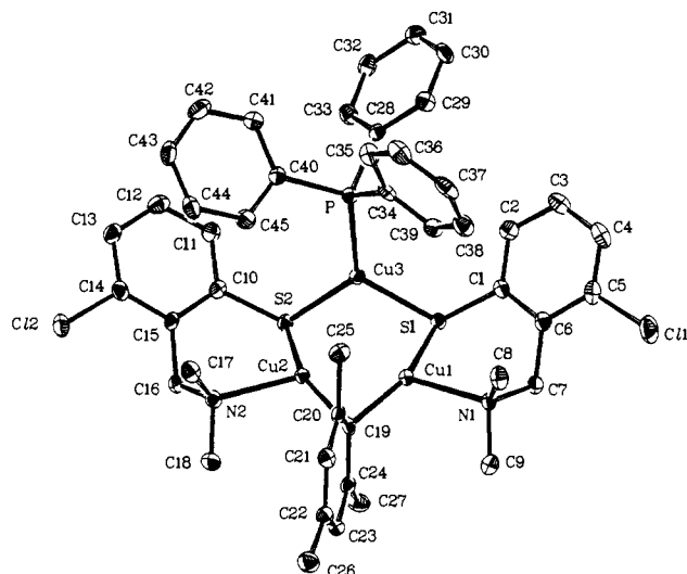
Figure 2. ORTEP drawing of [\text{Cu}_3\{\text{SC}_6\text{H}_3(\text{CH}_2\text{NMe}_2)\text{-}2\text{-Cl-}3\}_2(\text{C}_6\text{H}_2\text{Me}_3\text{-}2,4,6)(\text{PPh}_3)] ( 9 ) (with the exclusion of the hydrogen atoms and the benzene molecule) with the atom-labeling scheme. Ellipsoids are contoured at the 50% probability level.
