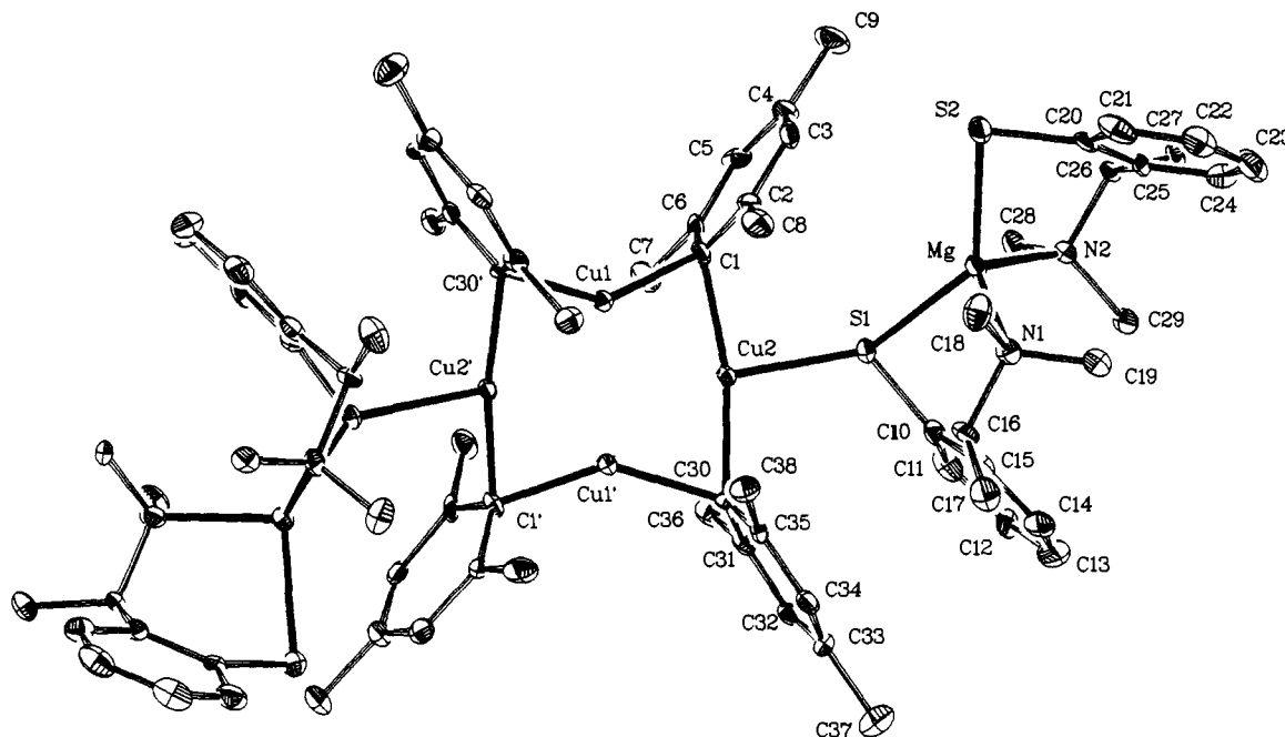
Figure 3. ORTEP drawing of [\text{Cu}_4\text{Mg}_2\{\text{SC}_6\text{H}_4(\text{CH}(\text{Me})\text{NMe}_2)_2\}_4(\text{C}_6\text{H}_2\text{Me}_3\text{-}2,4,6)_4] ( 14 ) (with the exclusion of the hydrogen atoms and the toluene molecule) with the atom-labeling scheme. Ellipsoids are contoured at the 50% probability level.
